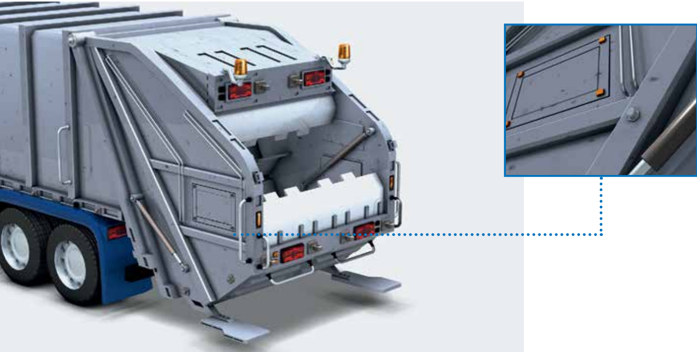
Garbage track. Intended specifically for demanding applications in moving machinery such as refuse-disposal trucks, earth-moving equipment and constriction and agricultural vehicles, E2AU sensors meet most severe regulatory standards for moving vehicles. These include e1 type approval (eMark) according to the European Automotive Directive 95/54/EC and electro-magnetic noise immunity up to 100 V/m according to ISO 11452-2.
