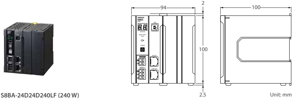
S8BA-24D24D240LF (240 W)
